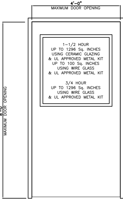
FIRE RATED SINGLE DOOR ONLY 1 LOUVER/WINDOW OPENING PER LEAF
