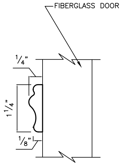
MOULDING APPLIQUE (MOULDING PROFILE MAY DIFFER) CHEMICALLY BONDED TO DOOR FACE
