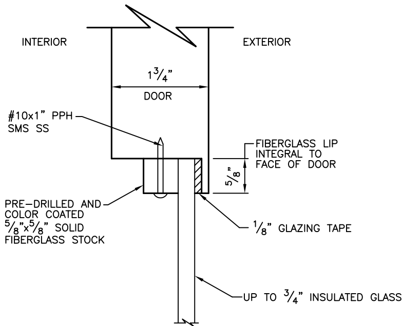
WINDOW SECTIONAL VIEW UP TO 3/4" GLAZING
