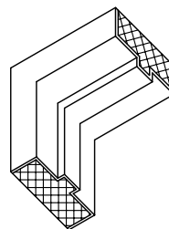
OPTION WF/T CHEMICALLY WELDED FACE/THROAT
