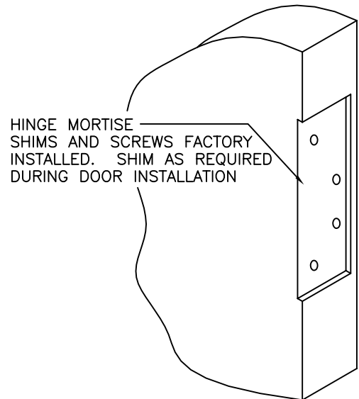
HINGE DETAIL
