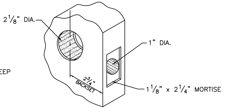
CYLINDRICAL LOCK DETAIL
