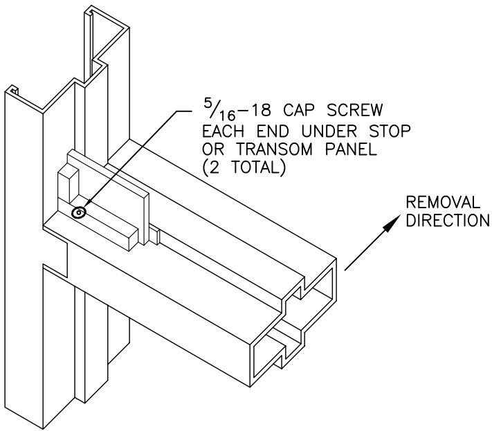
OPTION H1 INTERIOR VIEW LOOKING DOWN
